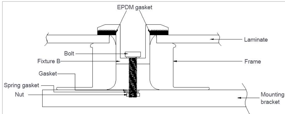
(Figure 7 Diagram of middle fixture)
