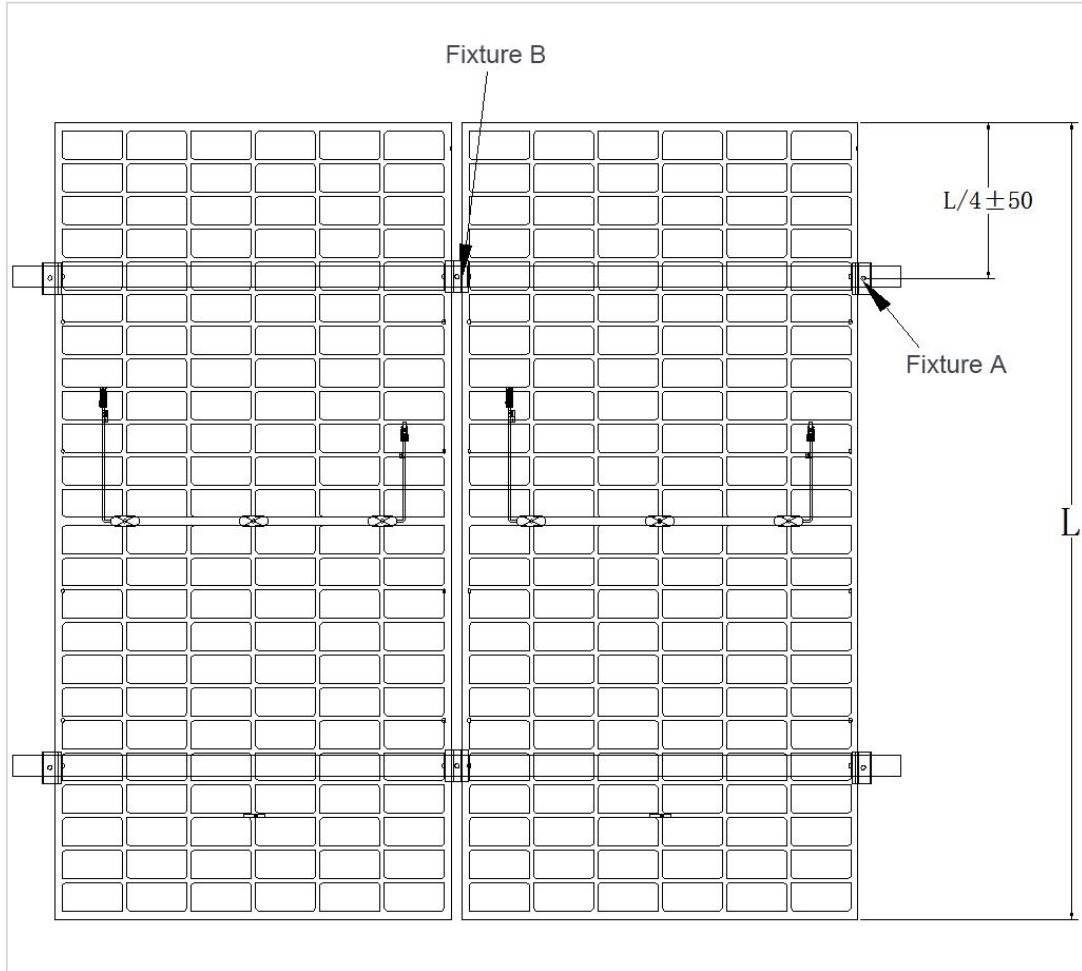
(Figure 5 Diagram of installation details)
