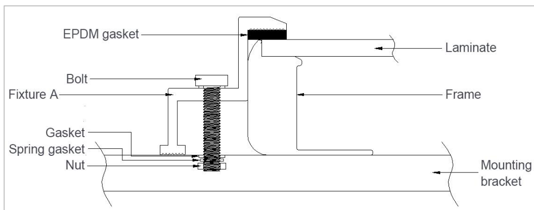
(Figure 6 Diagram of edge fixture)
