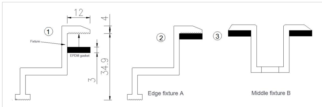
(Figure 3 Diagram of PV module fixture)
