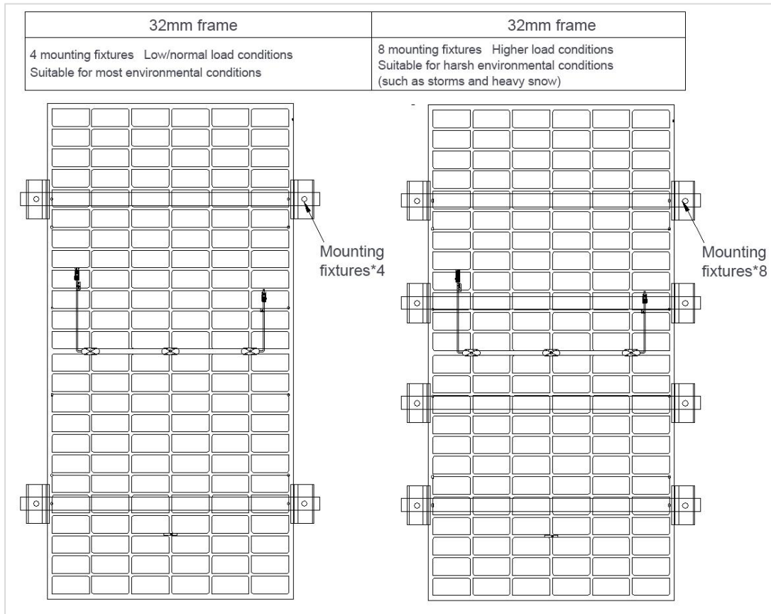
(Figure 4 Installation positions and corresponding load conditions)
