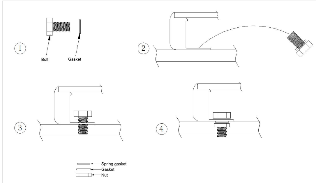
(Figure 1 Diagram of installation details)
